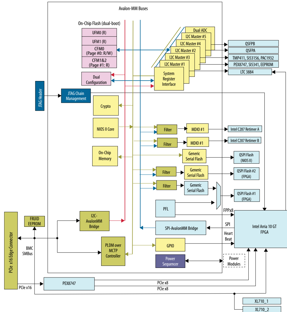
Figure 1. Block Diagram
