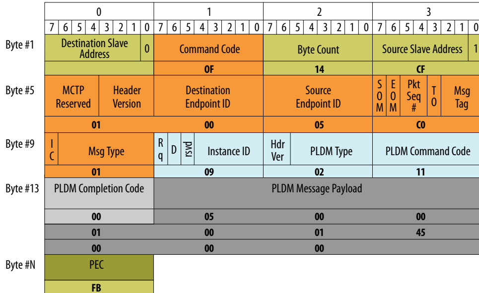
Figure 7. GetSensorReading Response Message Packet Fields
