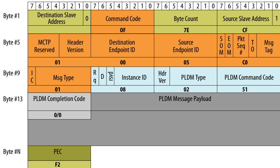
Figure 5. GetPDR Response Message Packet Fields
